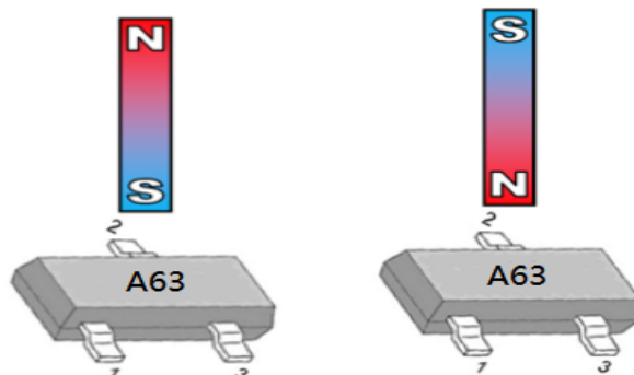
V OUT =低电压 V OUT =高电压 SOT23 (AH603)
